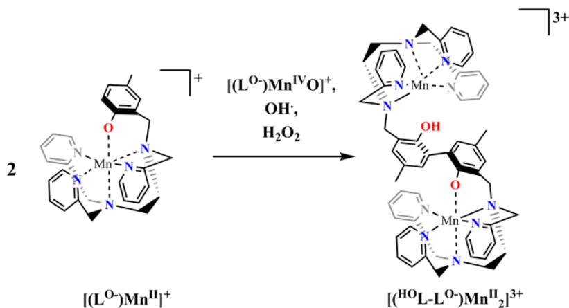
Scheme 3. Oxidative Coupling of Two Molecules of [(L^{O-})Mn^{II}]^+ Induced by [(L^{O-})Mn^{IV}O]^+ , OH^\bullet , or H_2O_2
