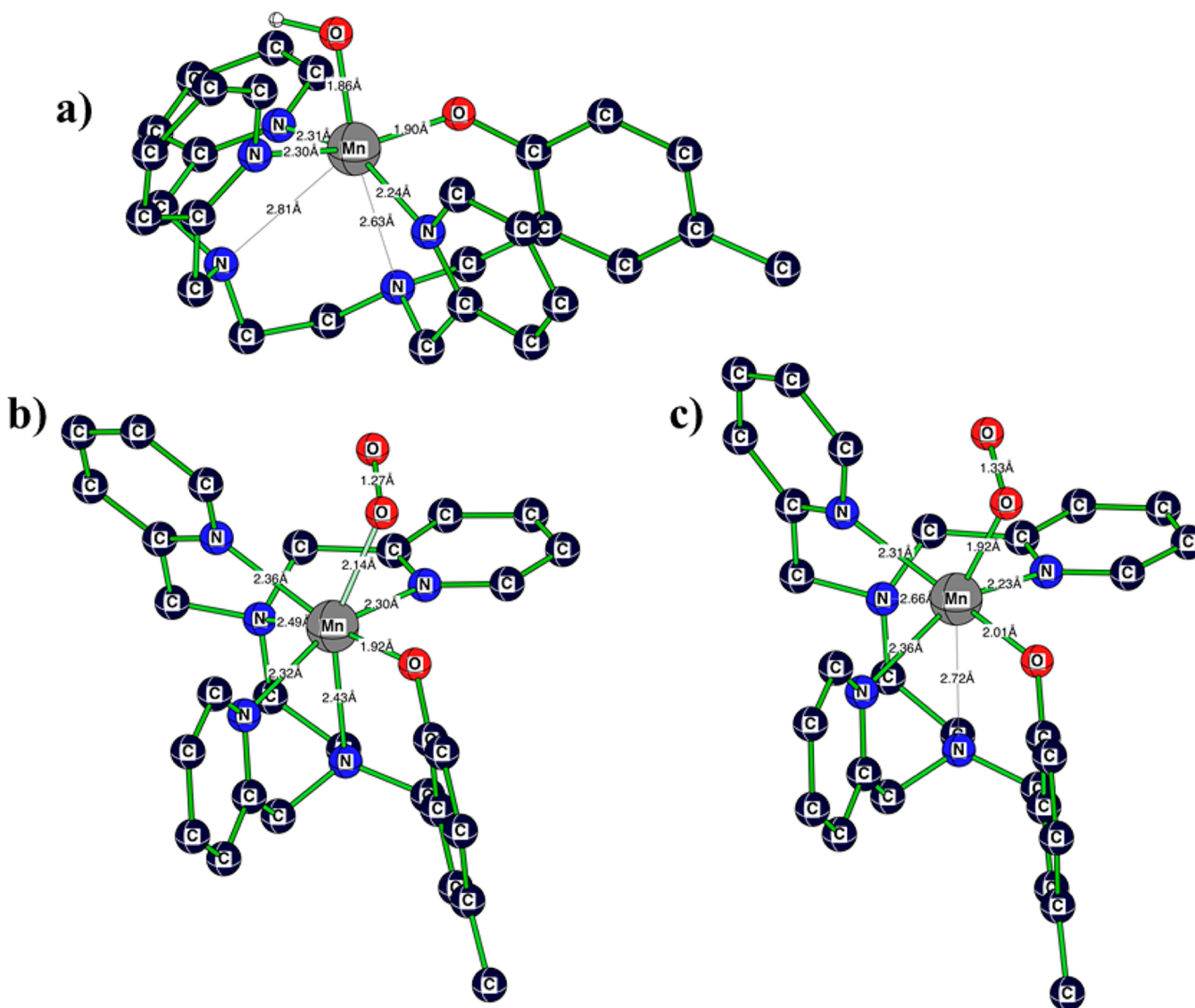
Figure 5. Calculated structures (UPW91PW91/def2svp) of (a) [(L^{O^-})Mn^{III}(OH^-)]^+ , (b) [(L^{O^-})Mn^{III}(O_2^{\bullet-})]^+ , and (c) [(L^{O^-})Mn^{III}(O_2^{2-})] . The hydrogen atoms of the polydentate ligand were omitted for clarity.
