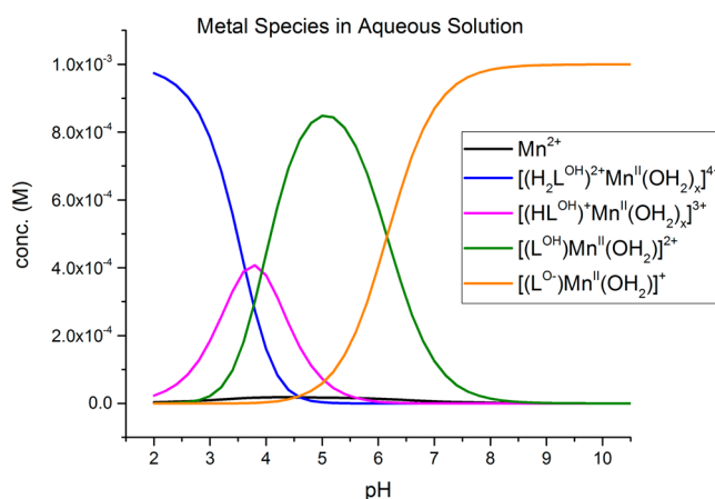
Figure 1. Species distribution of [(L OH )Mn II (solvent)](ClO 4 ) 2 (1) in aqueous solution at 21 °C.
